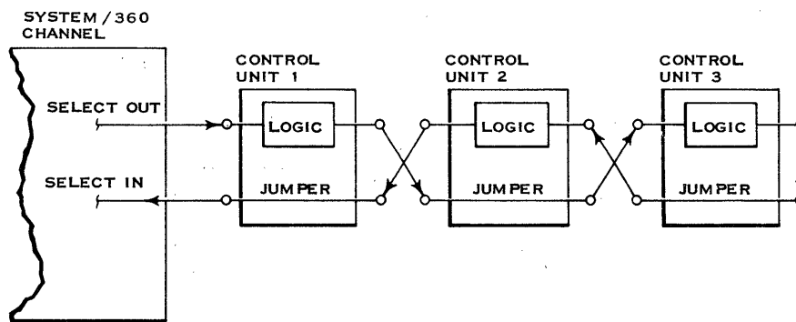
CONTROL UNIT PRIORITY
