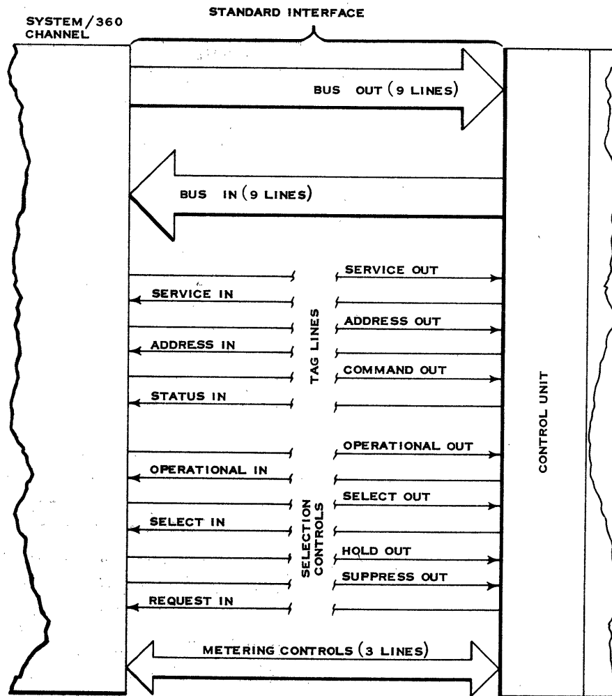
STANDARD INTERFACE LINES
